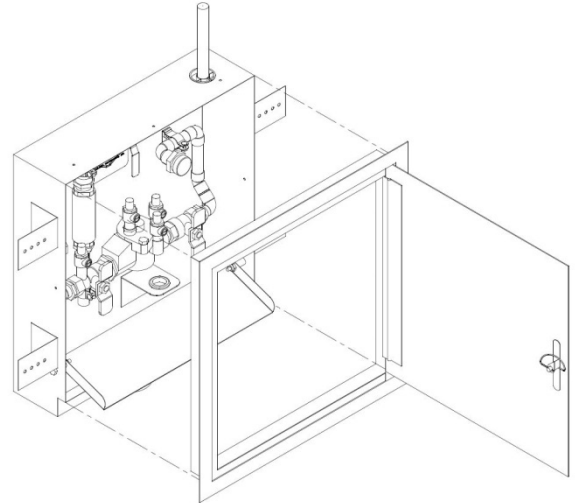
LEFT-FRONT VIEW
